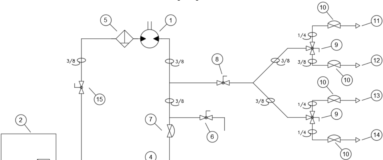
FIGURE 25, Plumbing Diagram
