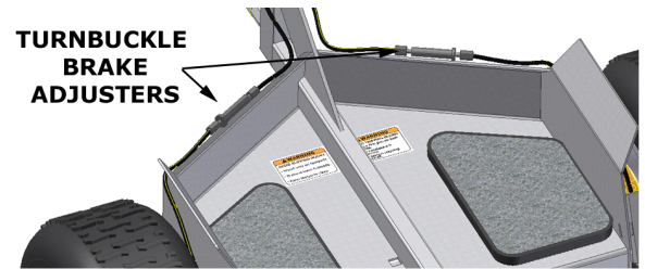
FIGURE 25 , Adjusting brakes
