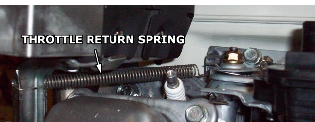
FIGURE 22 , Adjusting engine speed
