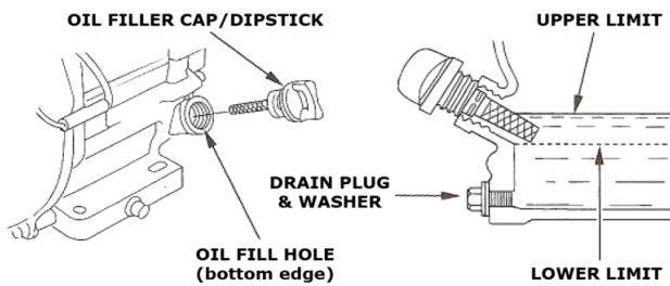
Check FIGURE 19 , Checking engine oil engine
