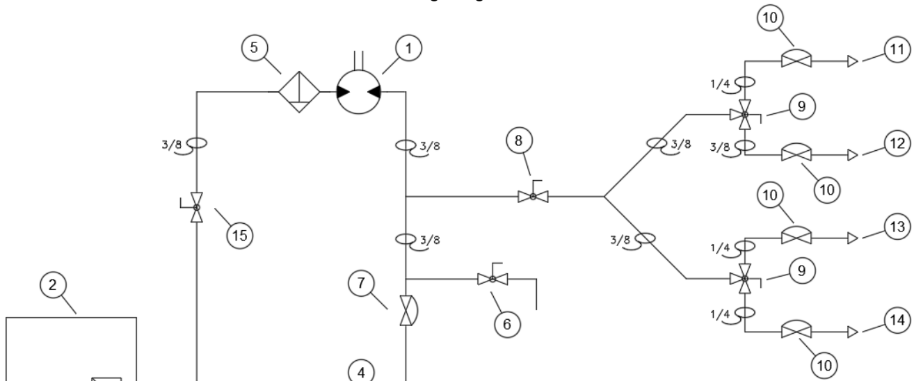
FIGURE 25, Plumbing Diagram
