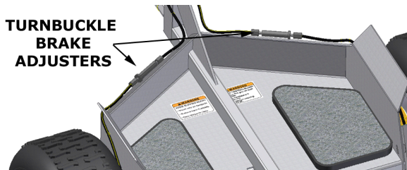
FIGURE 25 , Adjusting brakes
