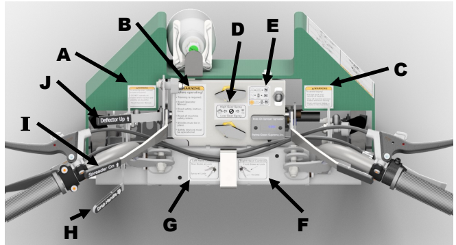
FIGURE 1, Dashboard Labels
