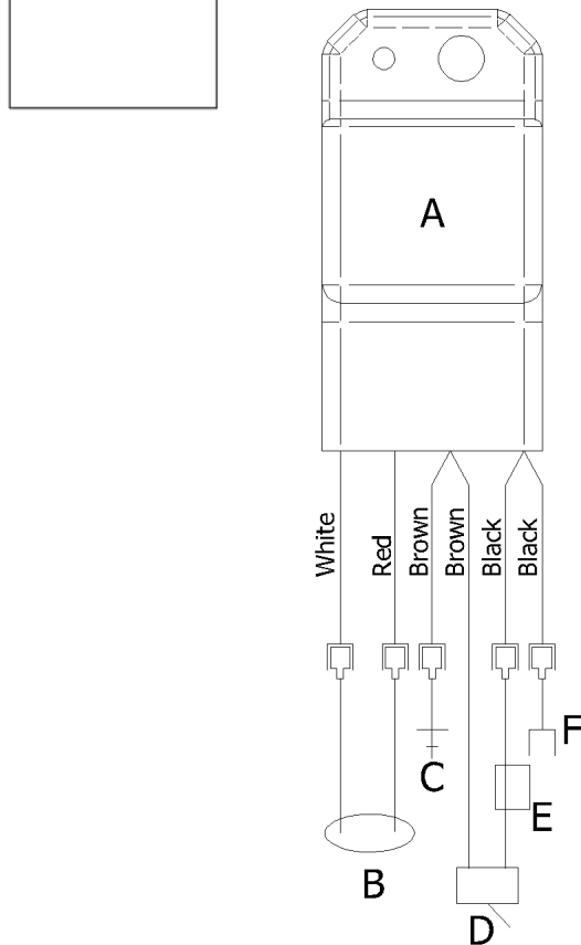
FIGURE 26, Wiring Diagram
