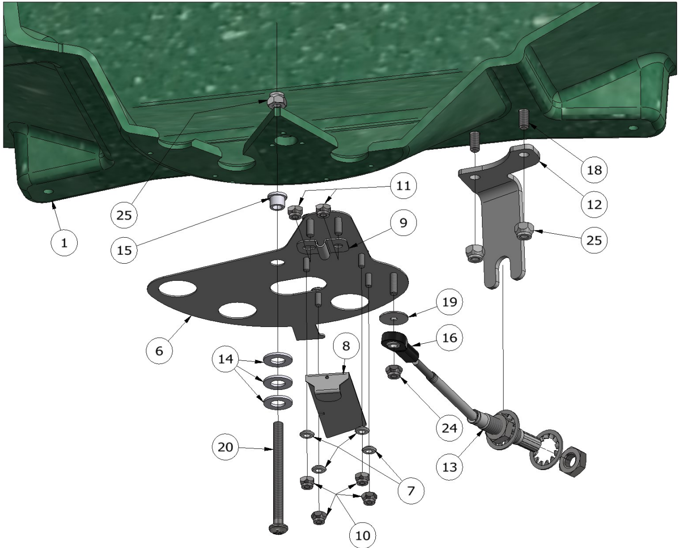
Fertilizer Rate, 3rd Hole Plates Fig. 28.1
