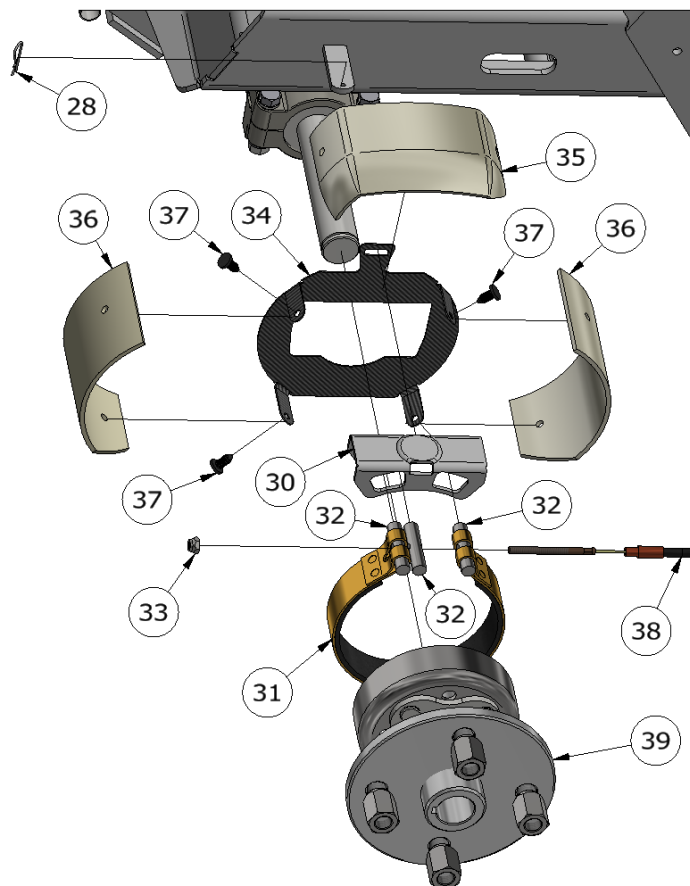
SS. Front Brake
