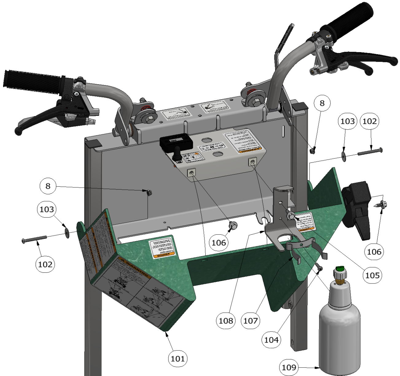
Handlebar Cover Fig. 29.12
