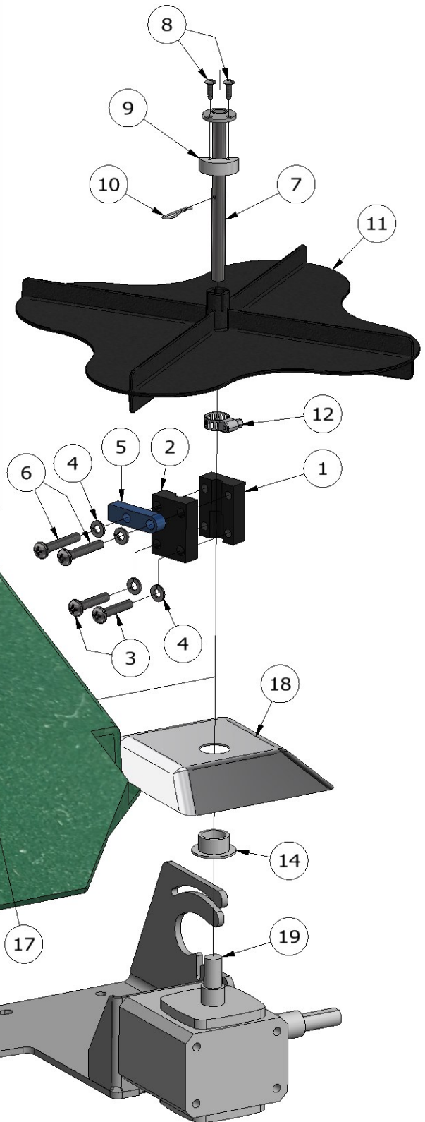
Spinner Group Fig. 28.8
