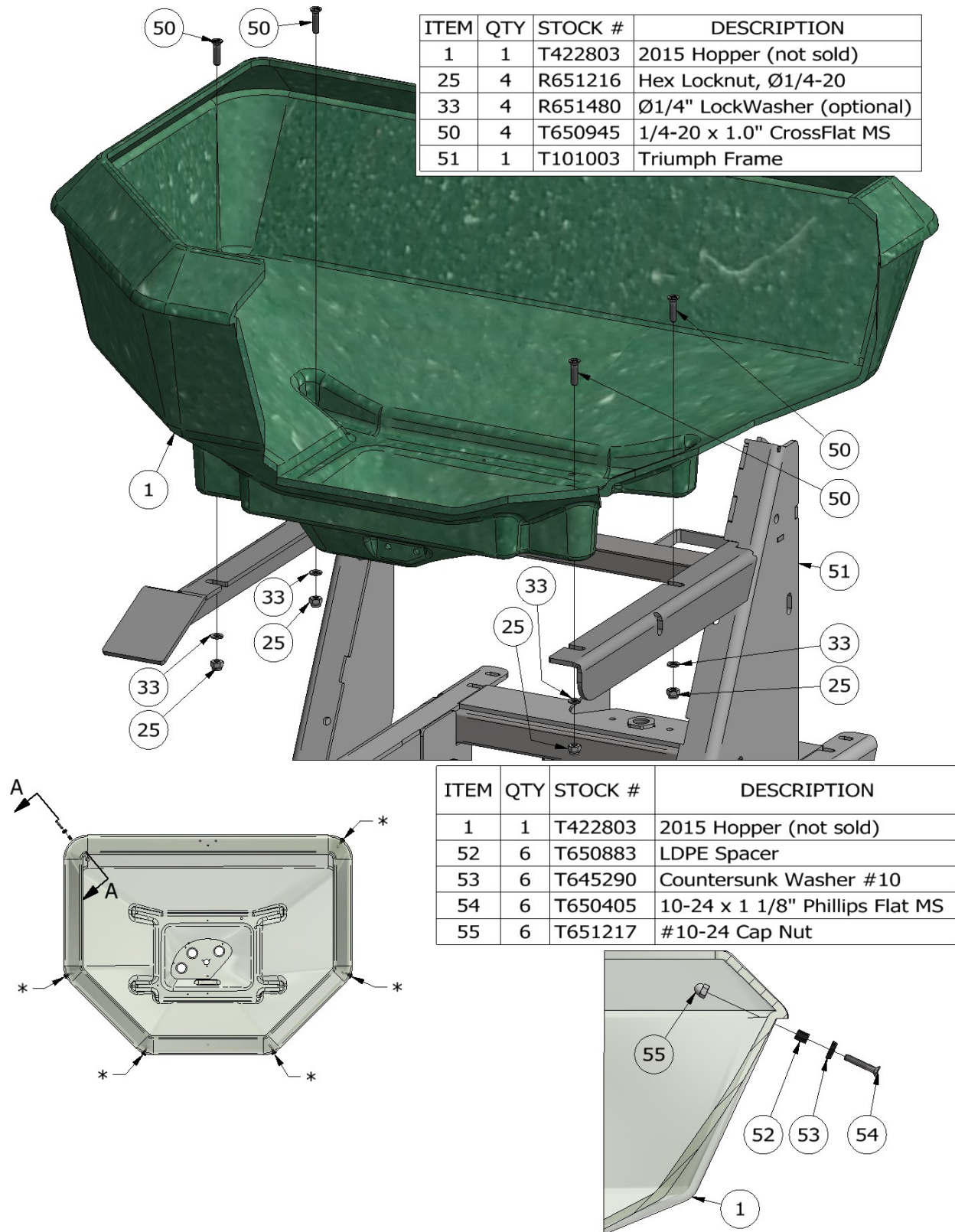
Hopper Mount Fig. 28.7
