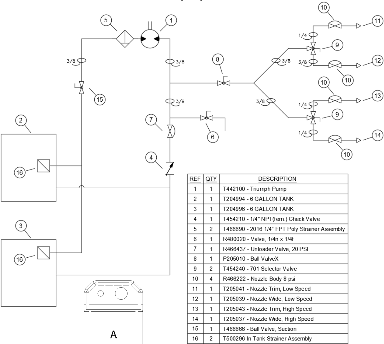
FIGURE 25, Plumbing Diagram
