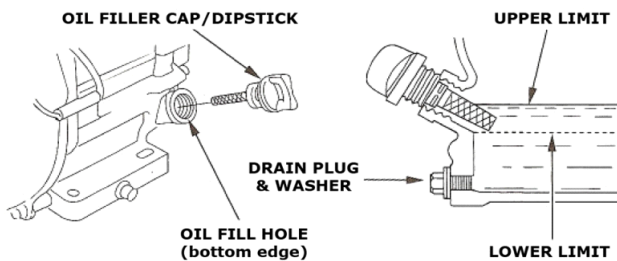
Check FIGURE 19 , Checking engine oil engine
