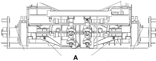
FIGURE 24, Grease points
