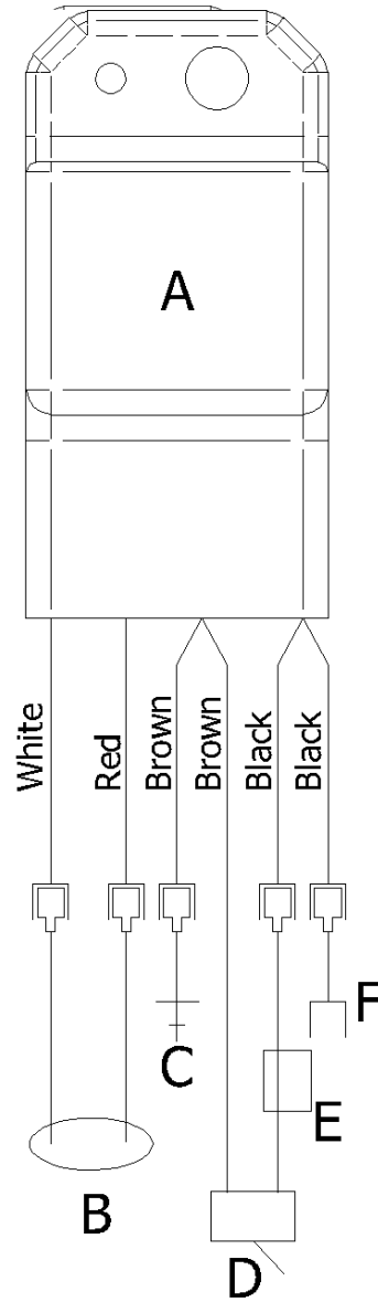
FIGURE 26, Wiring Diagram
