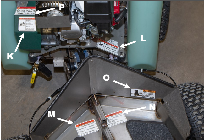
FIGURE 2, Rear Labels
